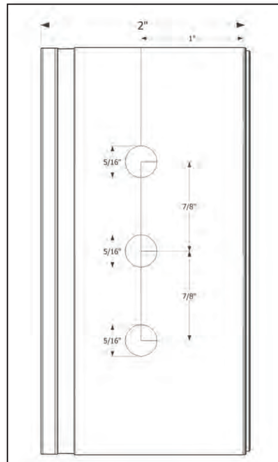
Screen Door Handle Drill Template
