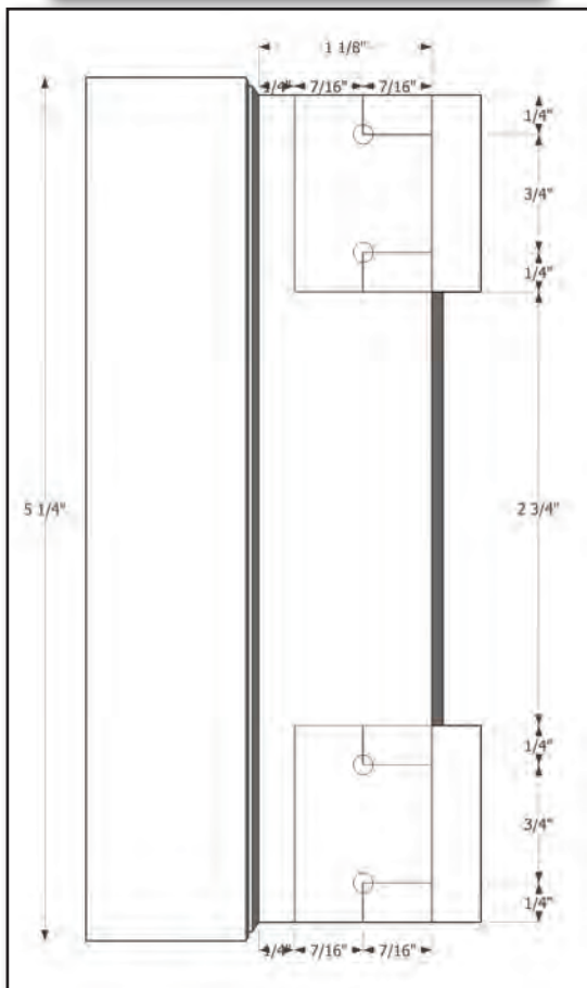
Screen Door Hinge to Jam Drill Template
