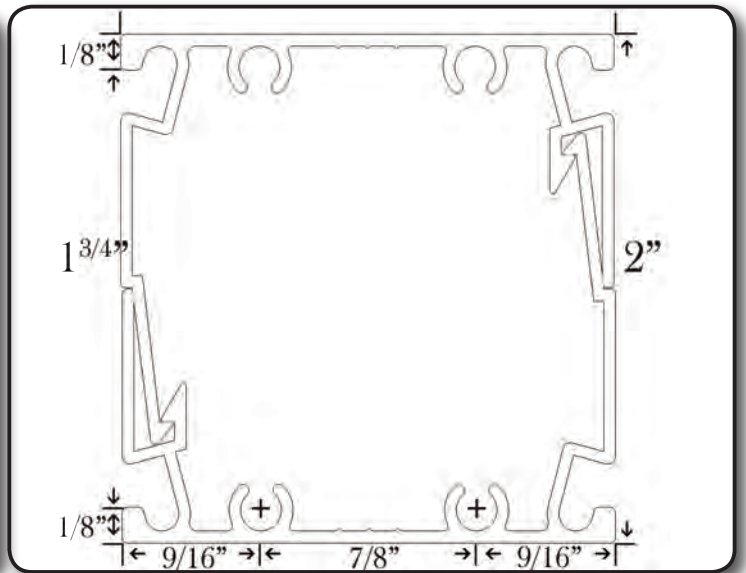
2x2 Self Mating Snap
